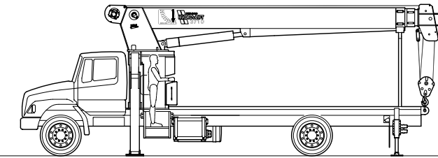
DECK MOUNT
