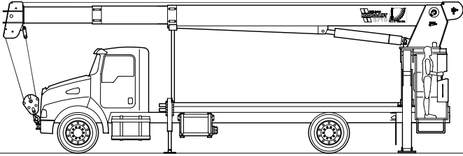
REAR MOUNT
